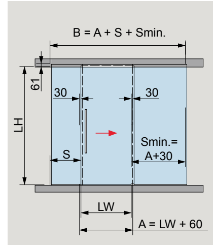
Single panel in ceiling, with two sidelights
