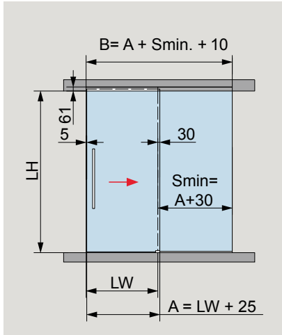
Single panel with sidelight, running / closing on 90° wall
