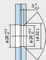
Glass thickness
