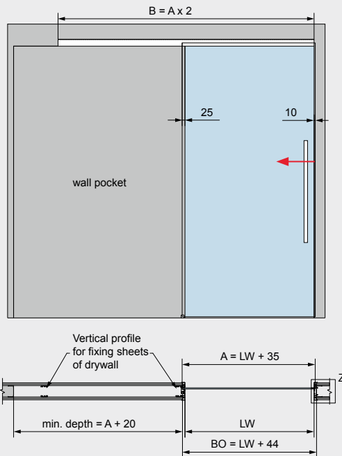
Fig. shows left opening (DIN right)
