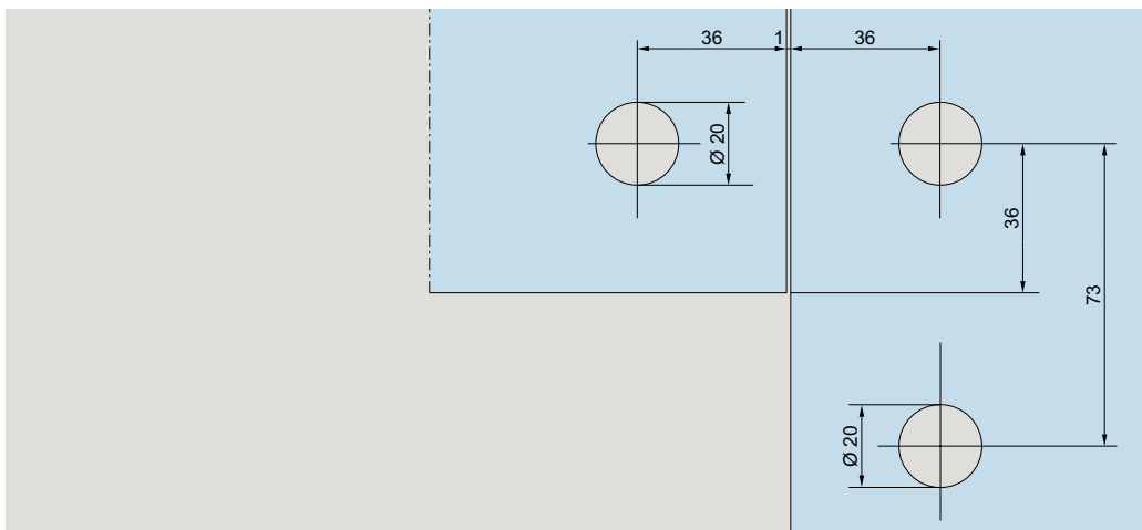
PT 60 Connectors for overpanels and sidelights
